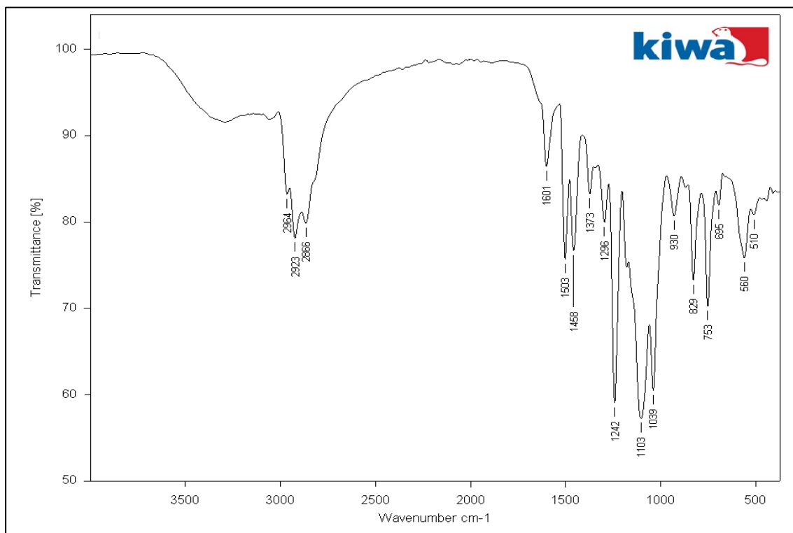
Picture 1: Infrared spectrum of ETS Aqua Primer , component A
