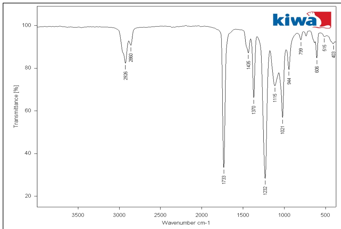
Picture 8: Infrared spectrum of ETS Eco Rapid , component A
