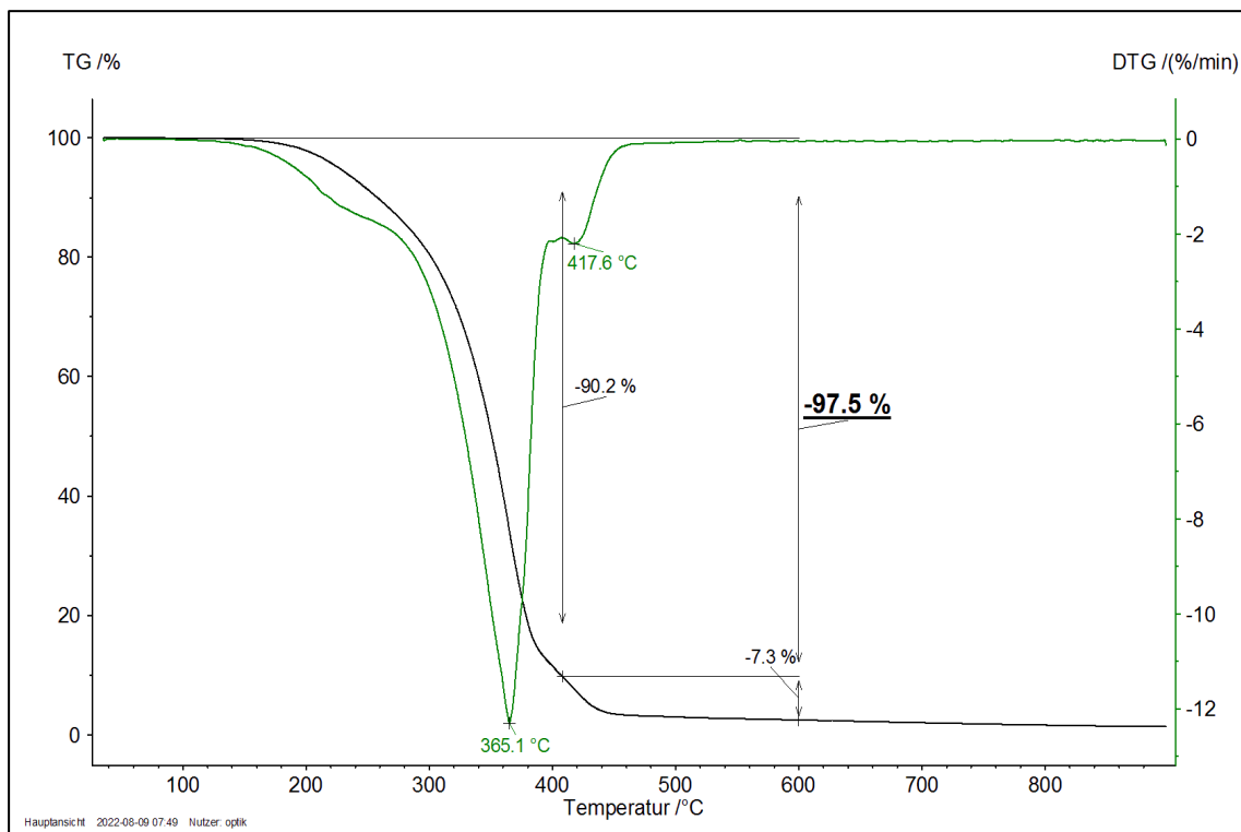
Picture 4 Thermogram of ETS Aqua Primer, component B
