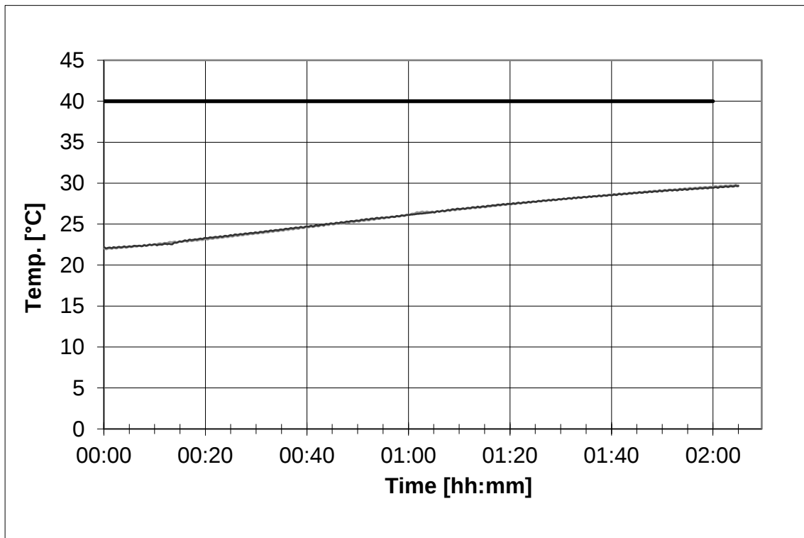
Picture 7: Potting/processing time of ETS Aqua Primer
