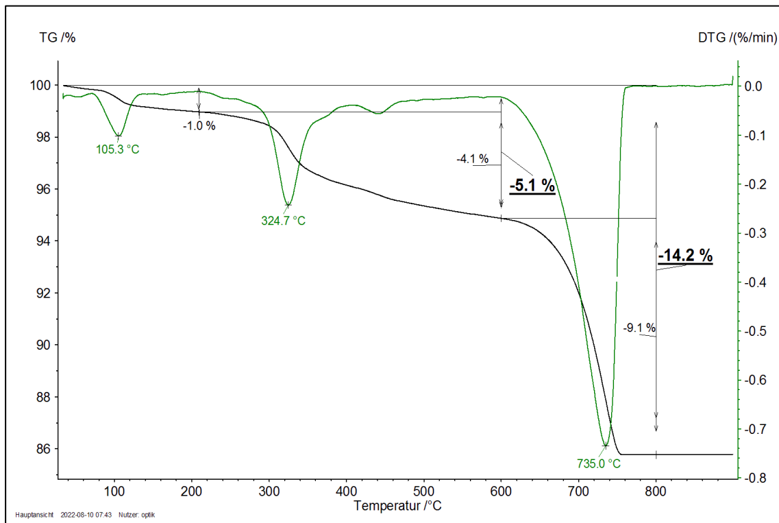
Picture 9: Thermogram of ETC Eco Rapid, component A
