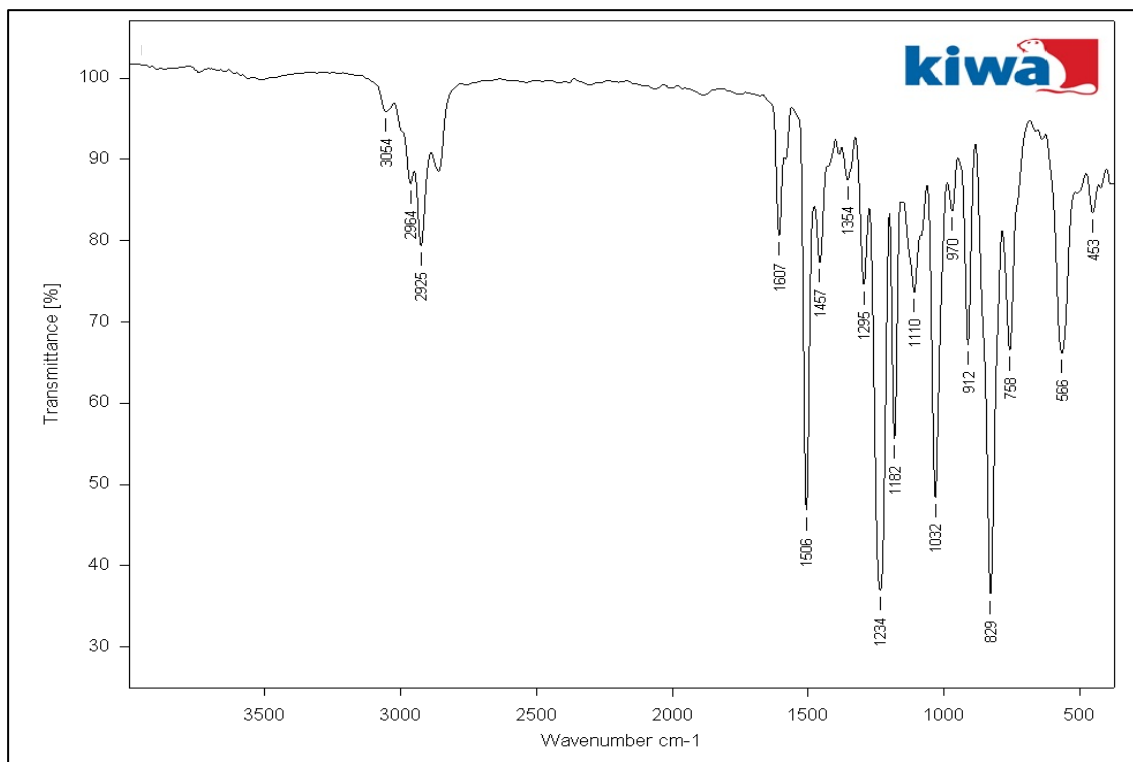
Picture 2: Infrared spectrum of ETS Aqua Primer , component B
