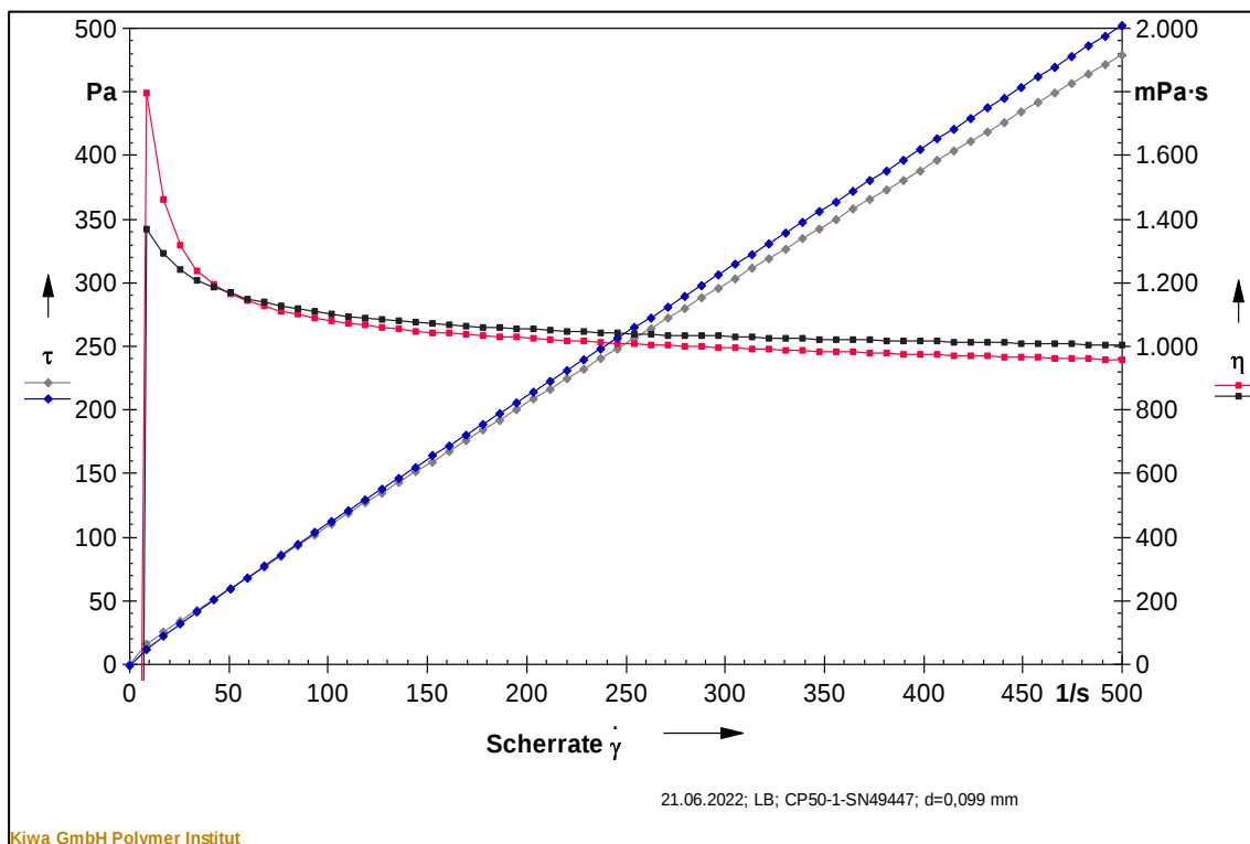
Picture 5: Flow and viscosity curve of ETS Aqua Primer, component A
