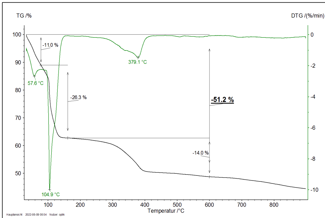
Picture 3 Thermogram of ETS Aqua Primer, component A
